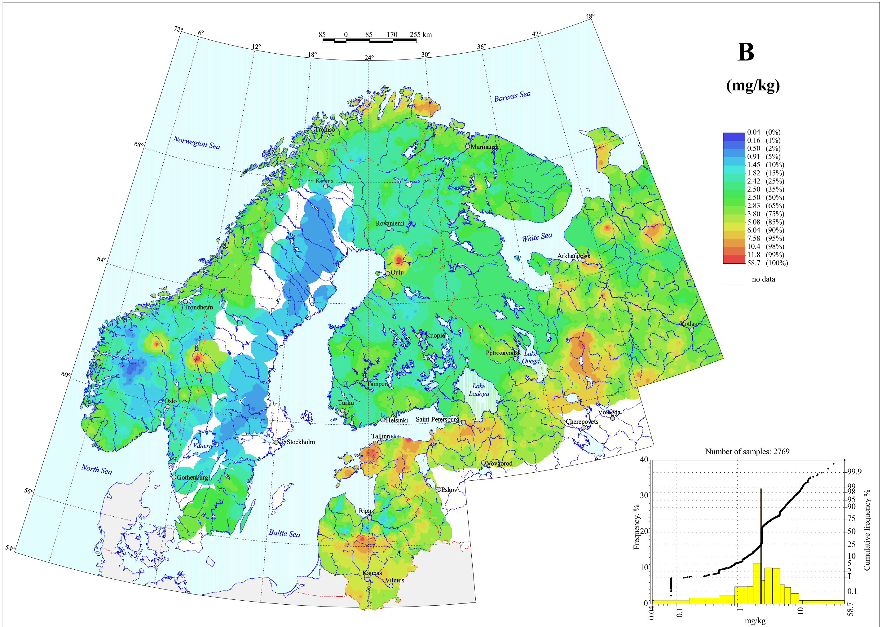
Boron in Organic Soil Layer, Total Content
